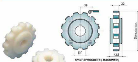
SPLIT SPROCKETS ( MACHINED )
